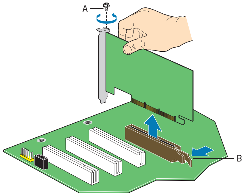
Figure 17. Removing an AGP Card
